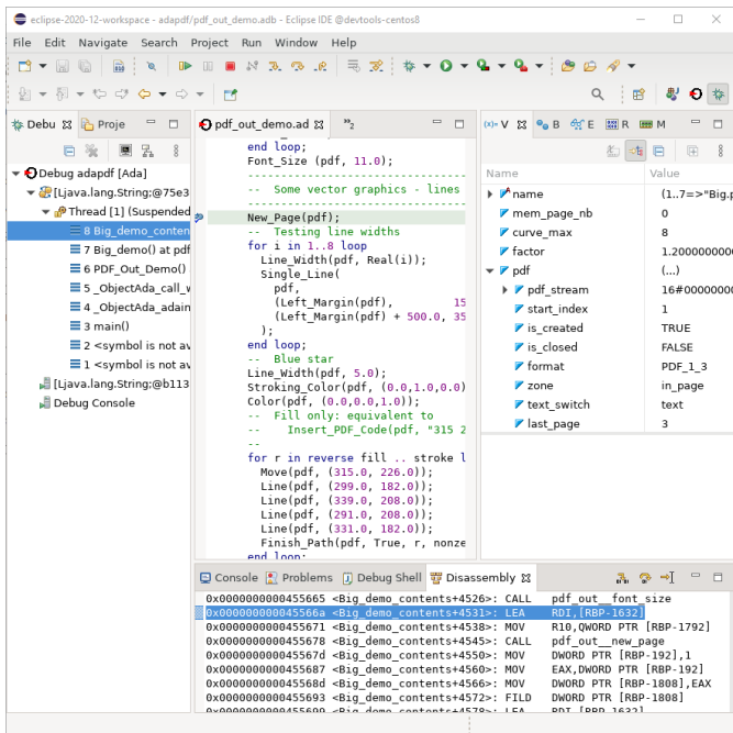
Using PTC ObjectAda Eclipse IDE Ada debugger
